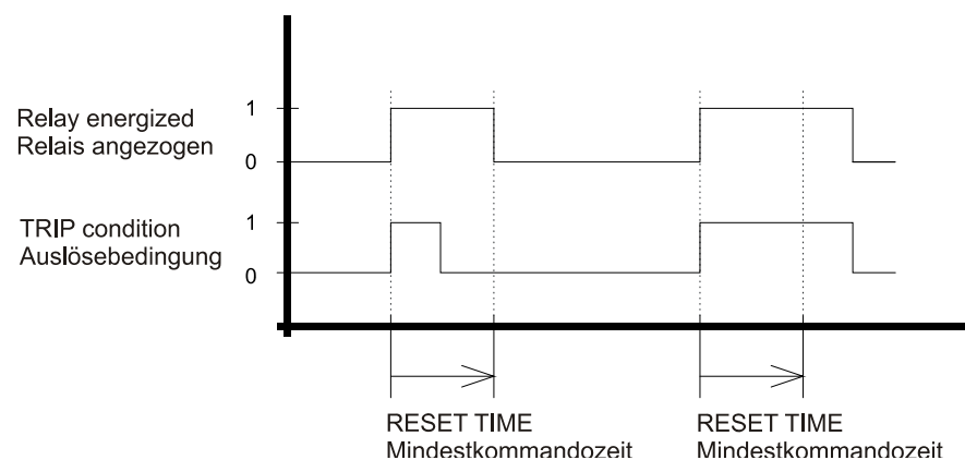
Figure 4.6.: Reset time
