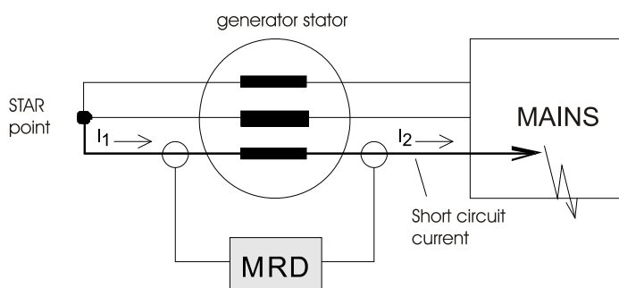
Figure 4.2: External fault
