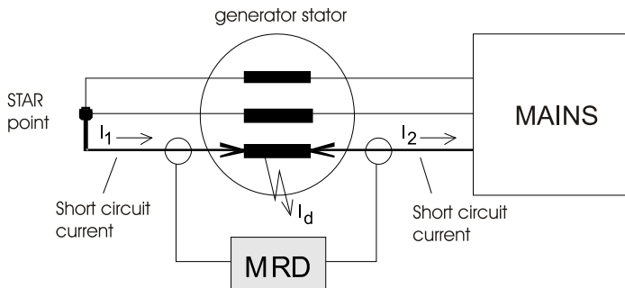
Figure 4.3: Internal fault (example of a short circuit fed from two sides)
