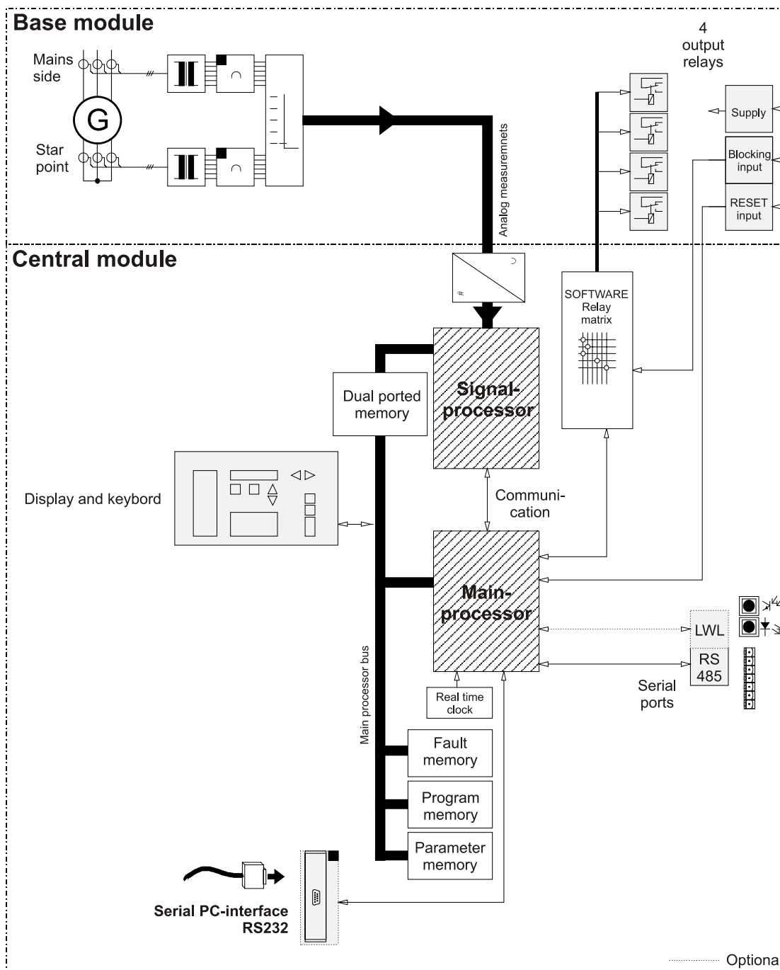
Figure 4.5: Block diagram
