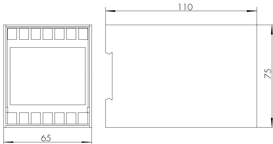
Fig. 5.1: Dimensional drawings
